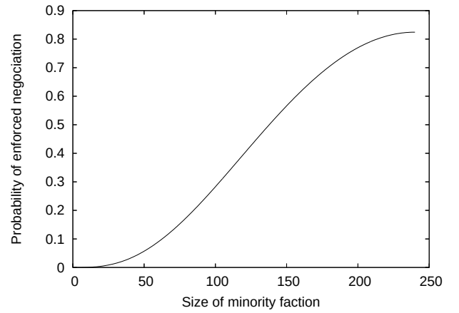
Figure 2. Probability that at some stage during the election process there is a college in which the factions have to negotiate
