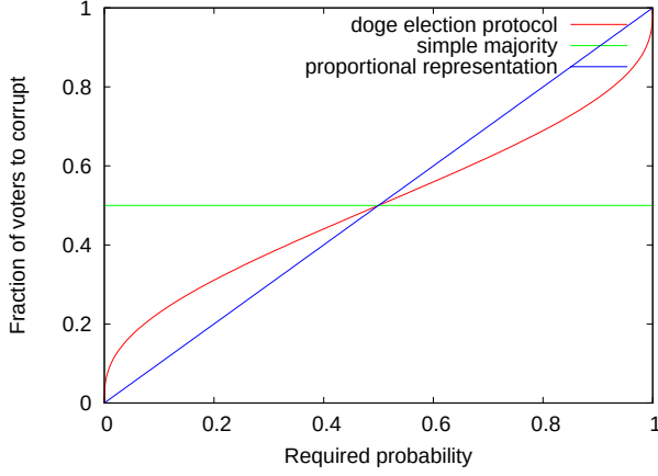
Figure 4. Fraction of voters in a large electorate that it is necessary for an attacker to corrupt to ensure a given probability of getting his candidate elected.
